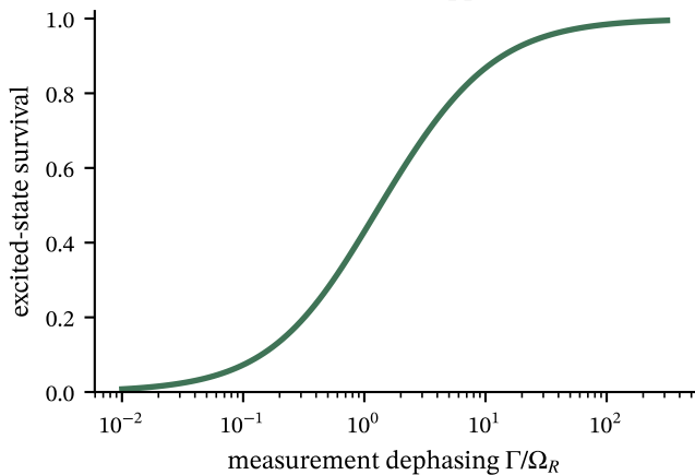
Quantum-Zeno suppression
